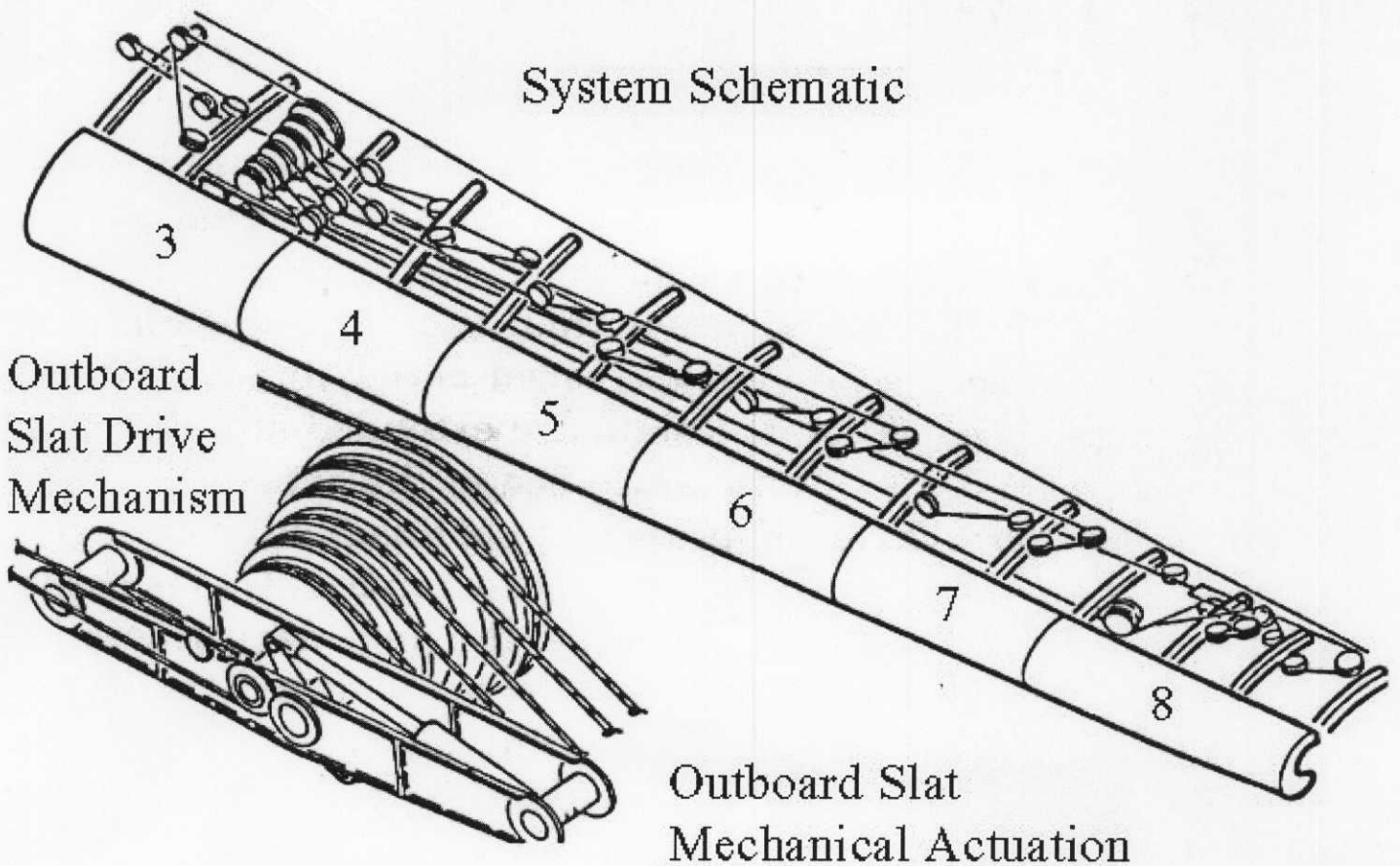
FIG. 15.3 Slat Mechanical Actuation
